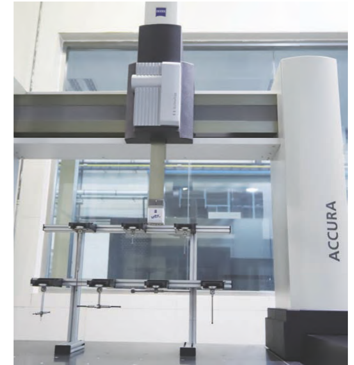
Three-coordinate Measure
