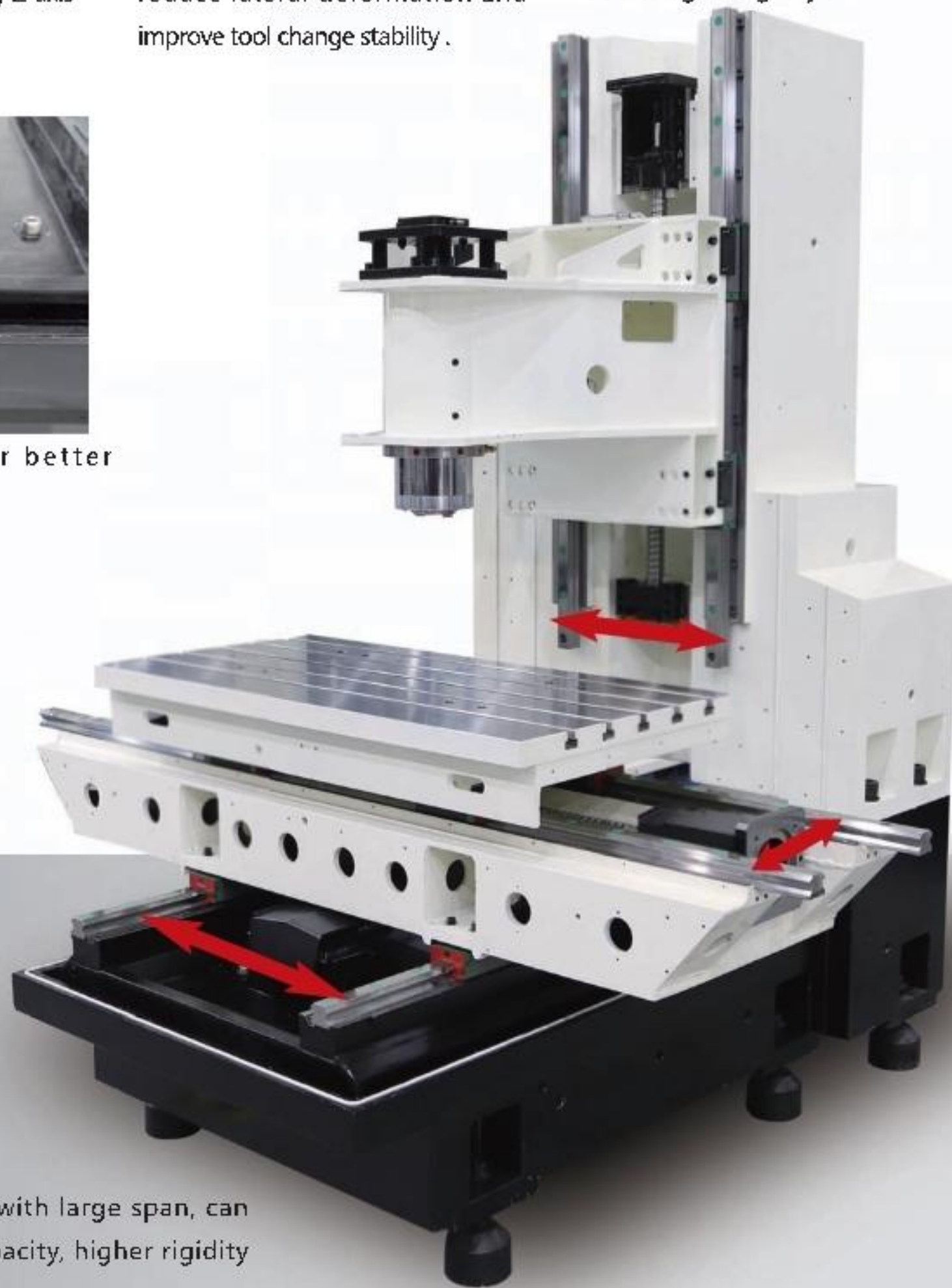
Headstock overhanging ratio 1:1 for higher rigidity .
