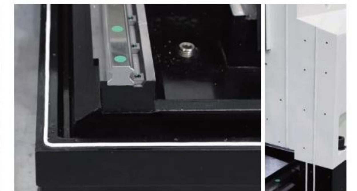
Pre-casted groove with sealing rubber strip to make machine cover non-leakage .
