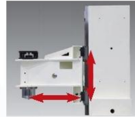
Headstock overhanging ratio 1:1 for higher rigidity .
