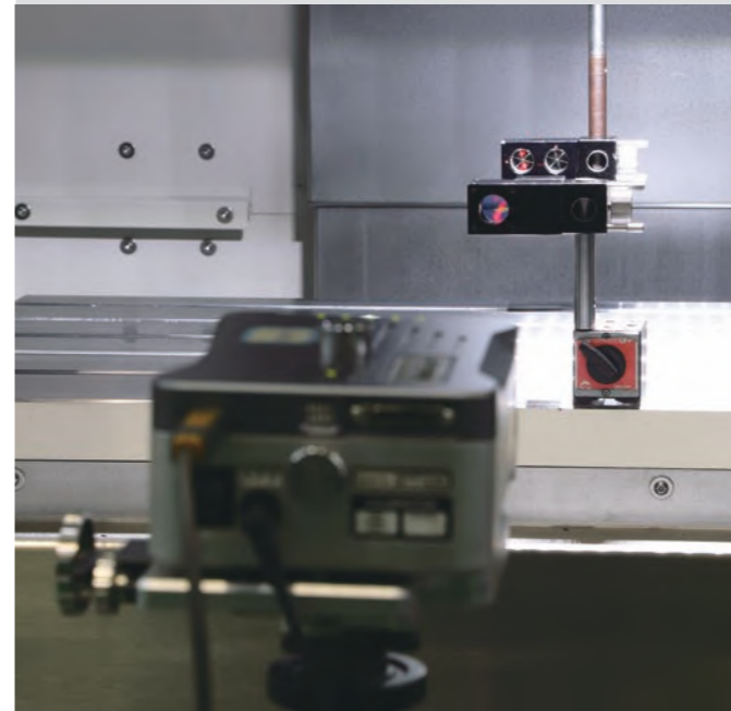
Laser Interferometer
