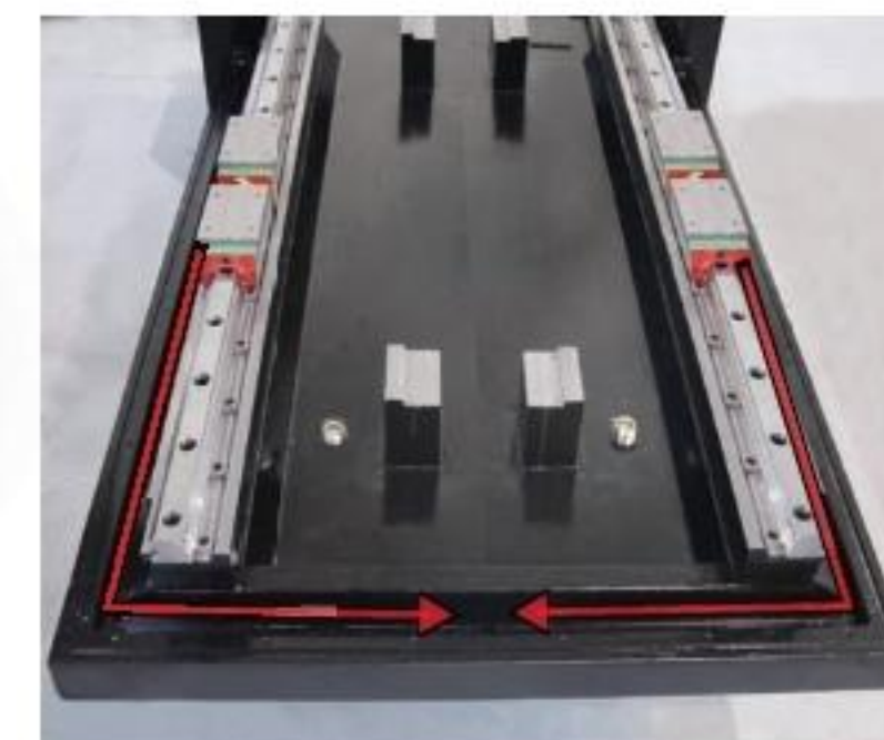
Water channel reserved on machine base, for cutting liquid backflow rather than overflow .
